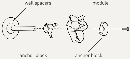
WALL ANCHORING
